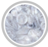
Quartz
